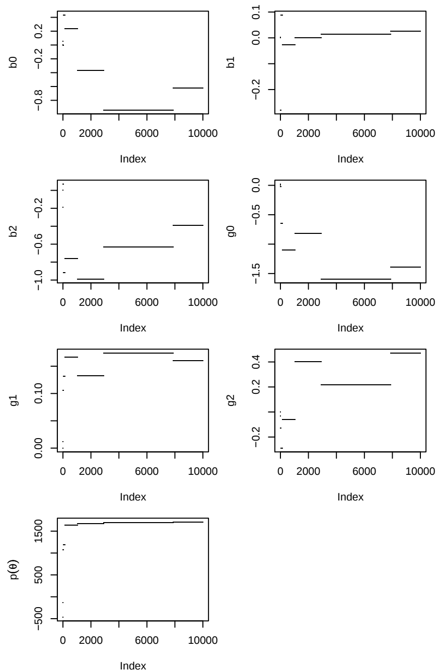
Figure 6.7: Trace plots of MCMC output from the pine cone code on page 363.
